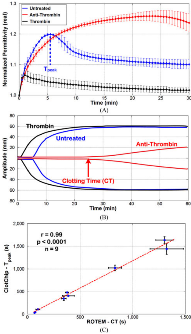
Fig. 7. Comparison of ClotChip T_{peak} and ROTEM CT parameters. (A) Time course of variation in \epsilon'_r at 1 MHz for an untreated whole blood sample and for the same sample treated with anti-thrombin as well as thrombin. (B) ROTEM profiles obtained for the three blood samples used in (A). The arrow shows the clotting time (CT) of the anti-thrombin-treated blood sample, defined as the time taken for the ROTEM profile to reach an amplitude of 2 mm. (C) A very strong positive correlation ( r = 0.99 , p < 0.0001 , n = 9 ) was observed between the ClotChip T_{peak} and ROTEM CT parameters. For all plots, error bars indicate duplicate measurements and are presented as mean \pm standard error of the mean (SEM).
