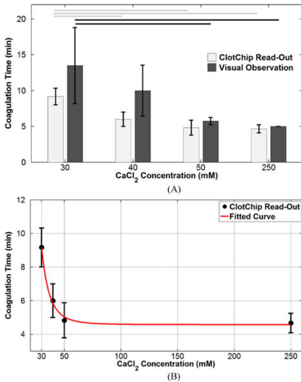
Fig. 6. Variation in coagulation time induced by changes in \text{CaCl}_2 concentration. (A) Bar graph comparing the ClotChip readout parameter T_{peak} versus visual observation-based readings of the coagulation time for various \text{CaCl}_2 concentrations. Horizontal lines indicate statistically significant difference in coagulation time at different concentrations ( p < 0.05 ). (B) Fitted curve to the ClotChip readout parameter T_{peak} showing a power relationship between the coagulation time and \text{CaCl}_2 concentration ( R^2 = 0.8344 ). Error bars represent the standard deviation of measurements run in triplicate for each \text{CaCl}_2 concentration.
