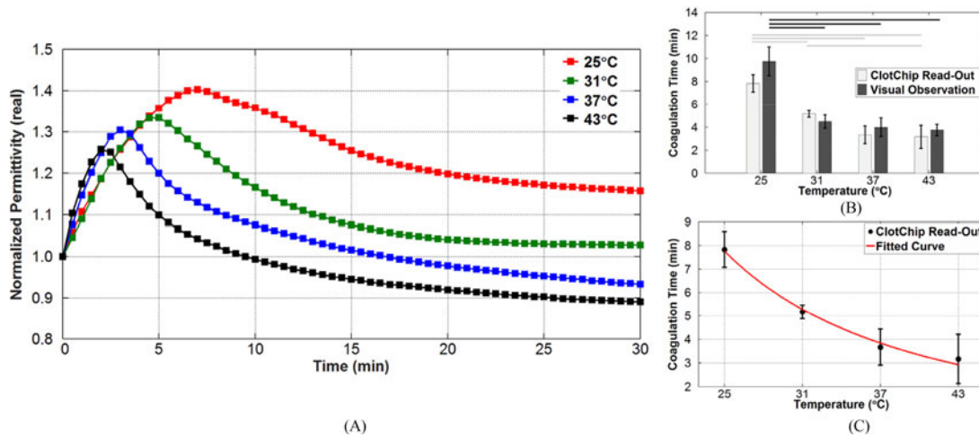
Fig. 5. Variation in coagulation time induced by a change in temperature. (A) Time course of variation in \epsilon_r' at 1 MHz for \text{CaCl}_2 -treated human whole blood at various temperatures. (B) Bar graph comparing the ClotChip readout parameter T_{peak} versus visual observation-based readings of the coagulation time for various temperatures. Horizontal lines indicate statistically significant difference in coagulation time at different temperatures ( p < 0.05 ). (C) Fitted curve to the ClotChip readout parameter T_{peak} showing a power relationship between the coagulation time and temperature ( R^2 = 0.8876 ). Error bars represent the standard deviation of measurements run in triplicate for each temperature.
