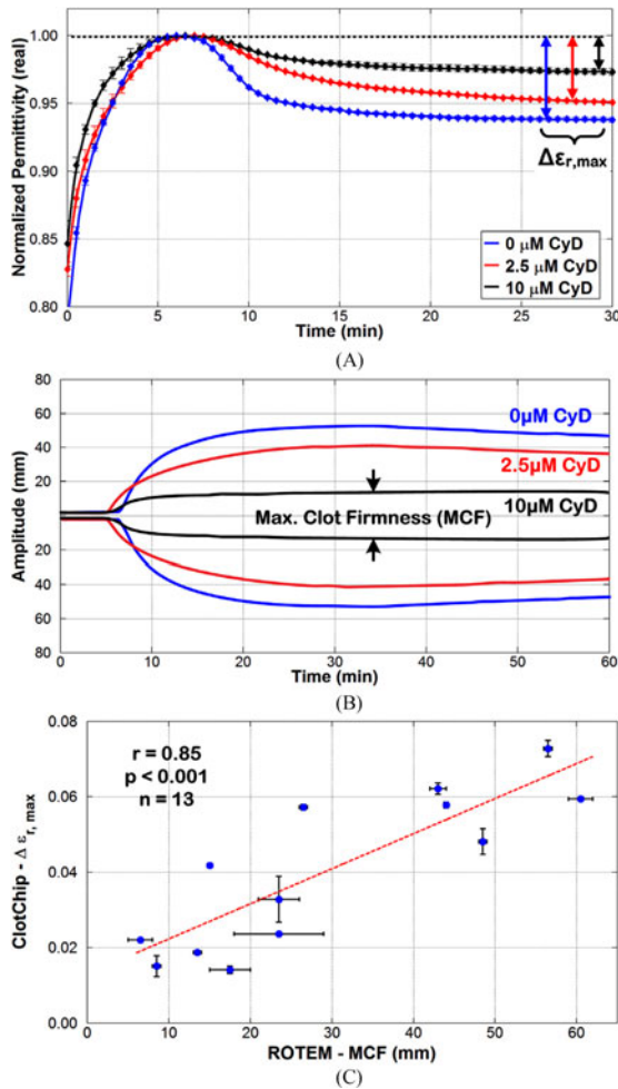
Fig. 8. Comparison of ClotChip \Delta\epsilon_{r,max} and ROTEM MCF parameters. (A) Time course of variation in \epsilon'_r at 1 MHz for an untreated whole blood sample (CyD concentration of 0 \mu\text{M} ) and for the same sample treated with CyD concentrations of 2.5 \mu\text{M} and 10 \mu\text{M} . (B) ROTEM profiles obtained for the three blood samples used in (A). The arrows show the maximum clot firmness (MCF) of the 10 \mu\text{M} -CyD-treated blood sample. (C) A strong positive correlation ( r = 0.85 , p < 0.001 , n = 13 ) was observed between the ClotChip \Delta\epsilon_{r,max} and ROTEM MCF parameters. For all plots, error bars indicate duplicate measurements and are presented as mean \pm SEM.
