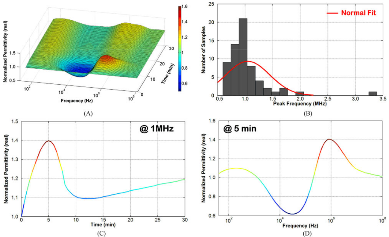
Fig. 3. Variation in \epsilon'_r of blood during coagulation. (A) Surface plot of the variation in \epsilon'_r of human whole blood versus time and frequency. (B) Histogram plot of the peak frequency for all tested blood samples. (C) 2D slice of the surface plot showing variation in \epsilon'_r versus time at 1 MHz. (D) 2D slice of the surface plot showing variation in \epsilon'_r versus frequency at 5 minutes.
