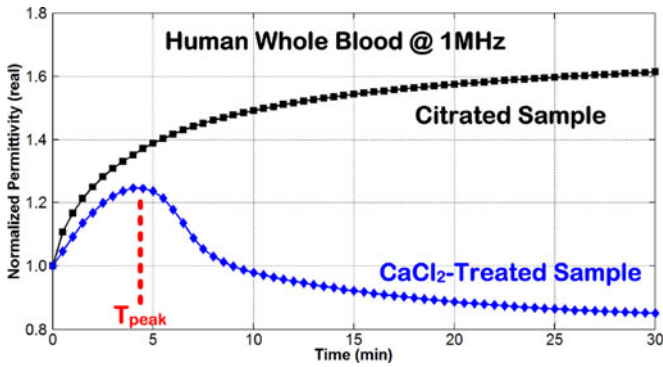
Fig. 4. Time course of variation in \epsilon'_r at 1 MHz for human whole blood without (black square) and with (blue diamond) coagulation initiated by the addition of \text{CaCl}_2 to a citrated (anticoagulated) blood sample [32].
