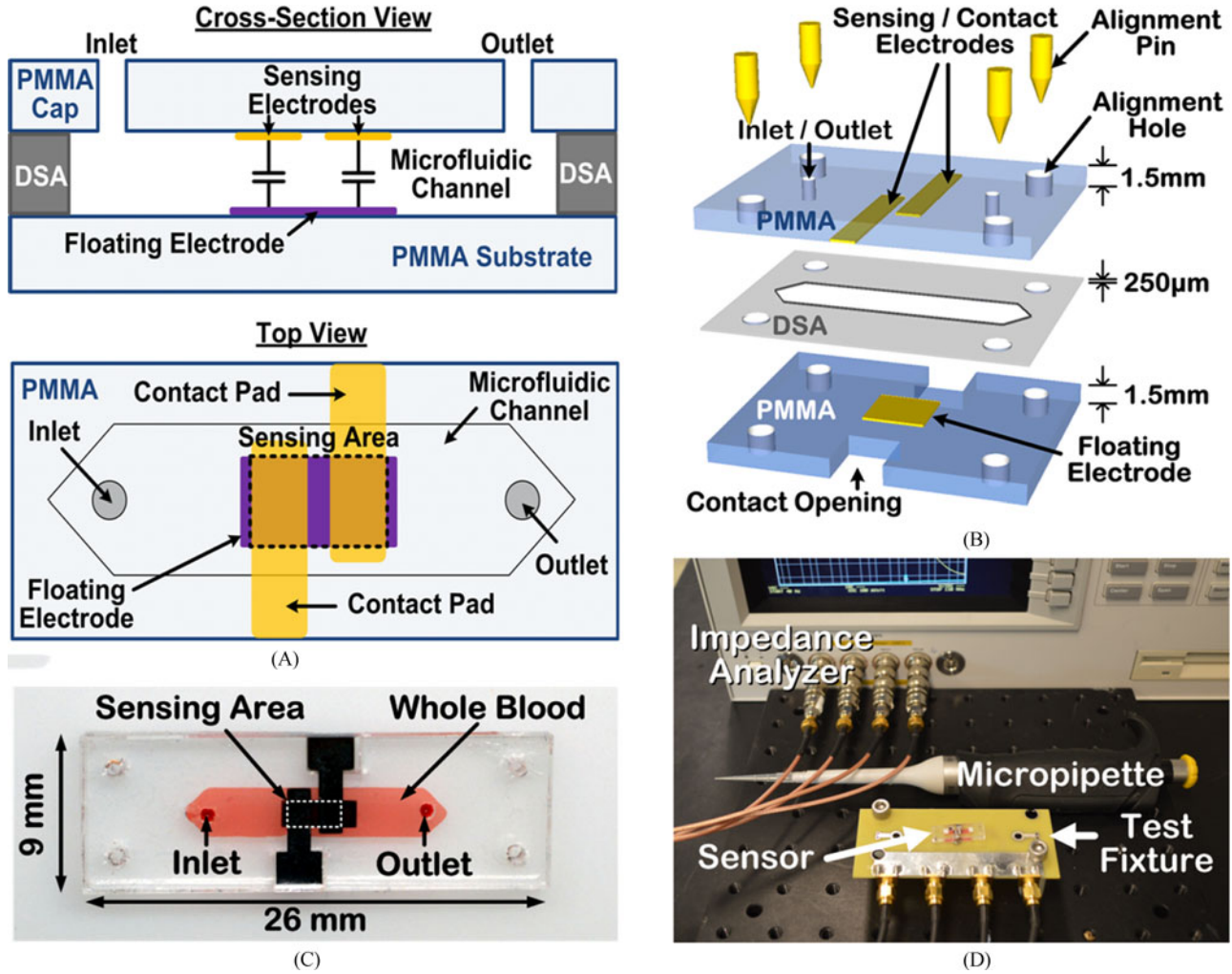
Fig. 2. Illustration of the ClotChip design and fabrication steps along with the experimental setup. (A) Cross-sectional and top views of the ClotChip. (B) ClotChip fabrication and assembly procedure. (C) Photograph of the fabricated ClotChip loaded with human whole blood as the MUT. (D) Photograph of the testing setup.
